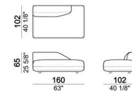
Central unit with right or left pouf
