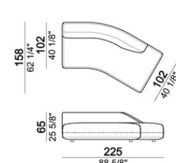
Central unit with right or left pouf and angle 30°
