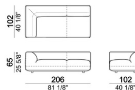
Right or left corner unit
