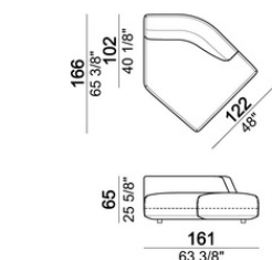
Right or left unit
