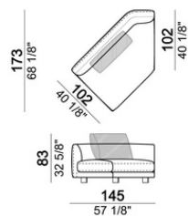
Central unit with right or left angle 45°
