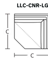
C: Grand 60", Studio 56", Micro 52"
