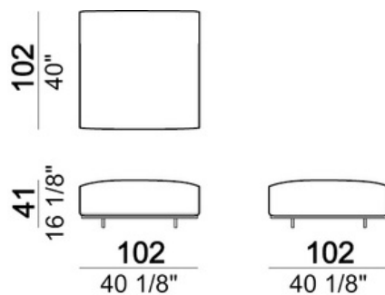
Central unit
