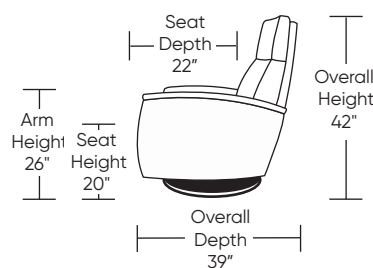
GOR-RV7-ST
