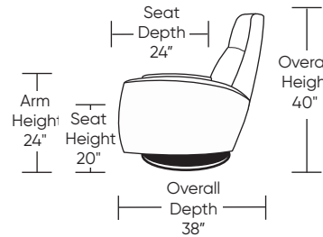
EVA-RV7-ST
