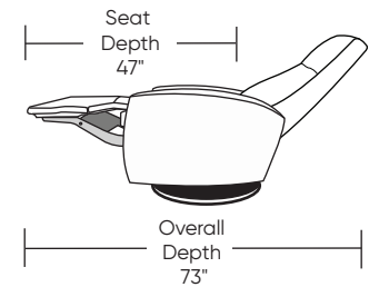
EVA-RV7-XT
