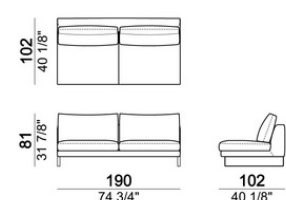
Central unit
